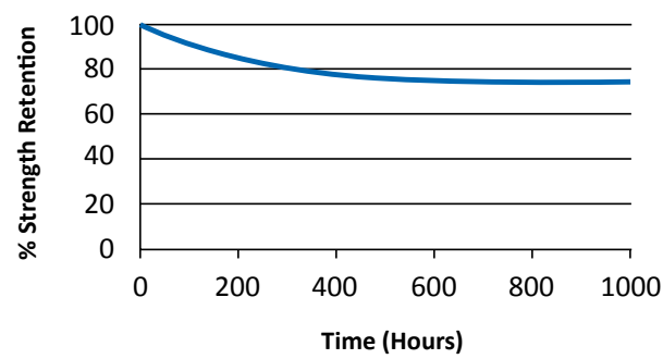
Thermal Ageing at 180°C (356°F)
